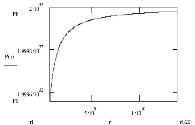
Figure 2. The radial distribution of the ether pressure for the Sun
