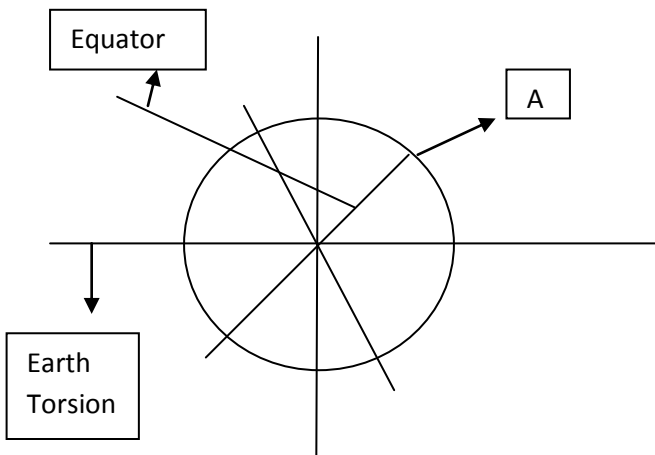
Fig. 4 Inclination of the Earth's equator
