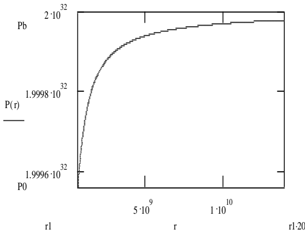
Fig. 2. Radial distribution of pressure of air for the Sun.
