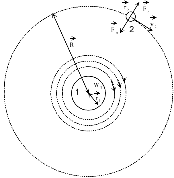
Fig. 1. Two-dimensional model of gravitational interaction of two bodies. Forces operating on a body 2 are specified. The F c -centrifugal force, F p -force of an attraction of a body 2 from a body 1, v 2 – the linear speed of a body 2 on an orbit, R – the radius of an orbit, r 1 – the radius of a body 1, r 2 – the radius of a body 2, w 1 – the angular speed of rotation of air on a surface of a body 1, m 2 – body weight 2.
