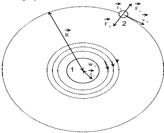
Fig.1. Two-dimensional model of the gravitational interaction between the two bodies.
