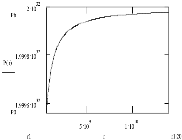
Fig.2. Radial distribution of ether pressure for the Sun.
