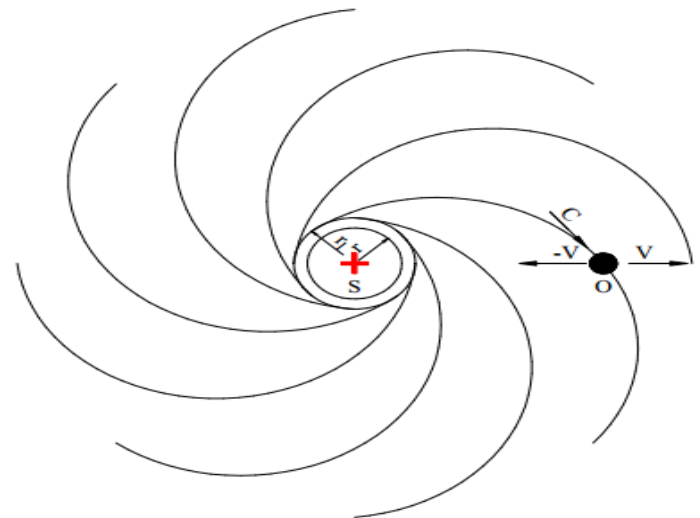
Fig. 1. S - light source (the atom), O - observer, r - radius of the atom, r_1 - the radius of the orbit of the highest flux at his address in a calm state, prior to heating (at orbital velocity), v - relative velocity of removal or approximation between S and O, c - velocity of light vector.
